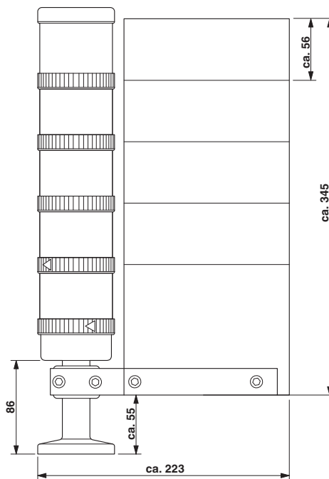
Dimensioned drawing
